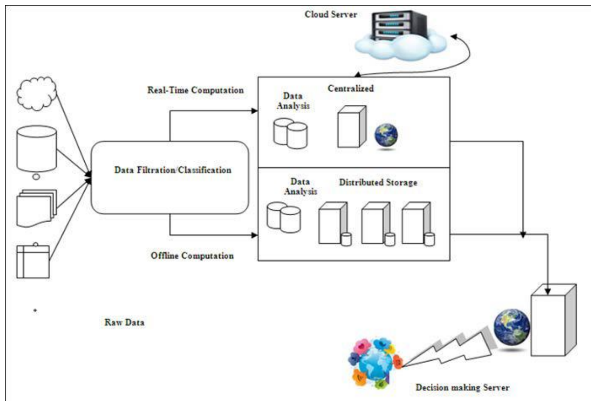
Figure 2. Real-time big data paradigm.
